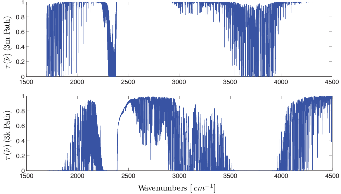
Figure 23. LBLRTM generated atmospheric transmittance profile for H_2O and CO_2 . Top panel represents transmittance through 3 meters of air. Bottom panel represents transmittance through 3 kilometers of air.
